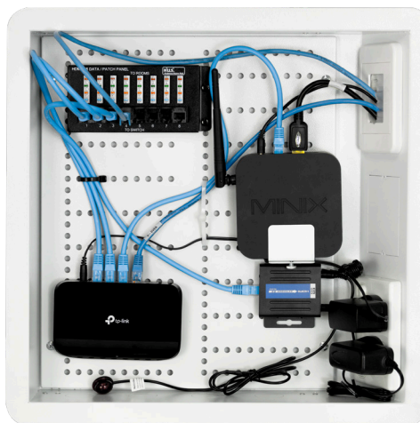
(05DRWBL Assembled)
